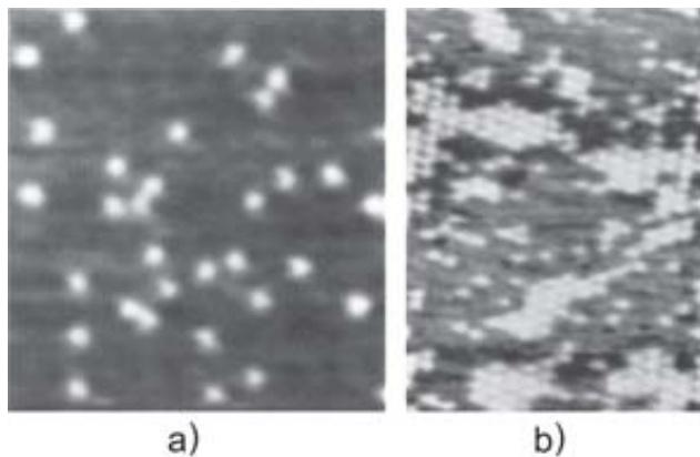
Figure 7. STM snapshots from O atoms adsorbed on a Ru(001) surface at T = 300 K [18]. a) very small coverage. b) higher coverage. In the lecture a short movie was presented showing the motion of the O atoms in real time.
