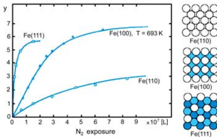
Figure 9. The variation of the relative coverage y of N atoms chemisorbed at 693 K at various Fe single crystal surfaces with exposure to gaseous N_2 [22] ( 1 \text{ L} = 1.33 \times 10^{-6} \text{ mbar} \cdot \text{sec} is about the exposure which would suffice to form a complete monolayer if each incident molecule would be adsorbed).
