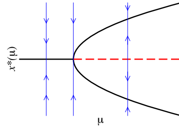
Fig. 12.19 Pitchfork bifurcation diagram.
