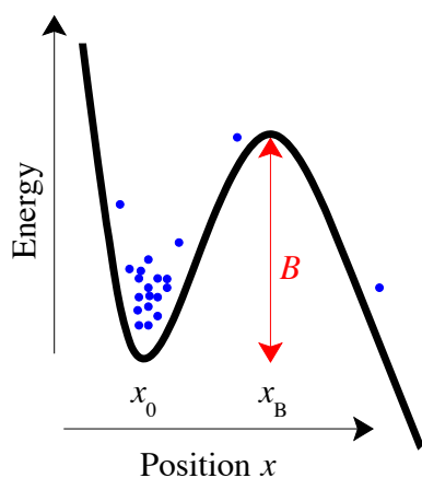
Fig. 6.7 Barrier-crossing potential.
