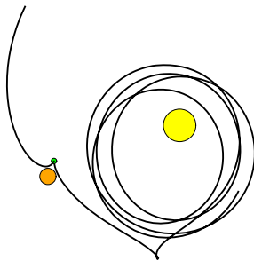
Fig. 4.6 The Earth's trajectory around the Sun if Jupiter's mass is abruptly increased by about a factor of 100.
