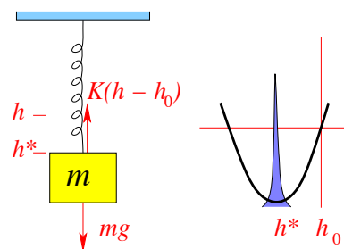
Fig. 6.5 A mass on a spring in equilibrium sits very close to the minimum of the energy.
